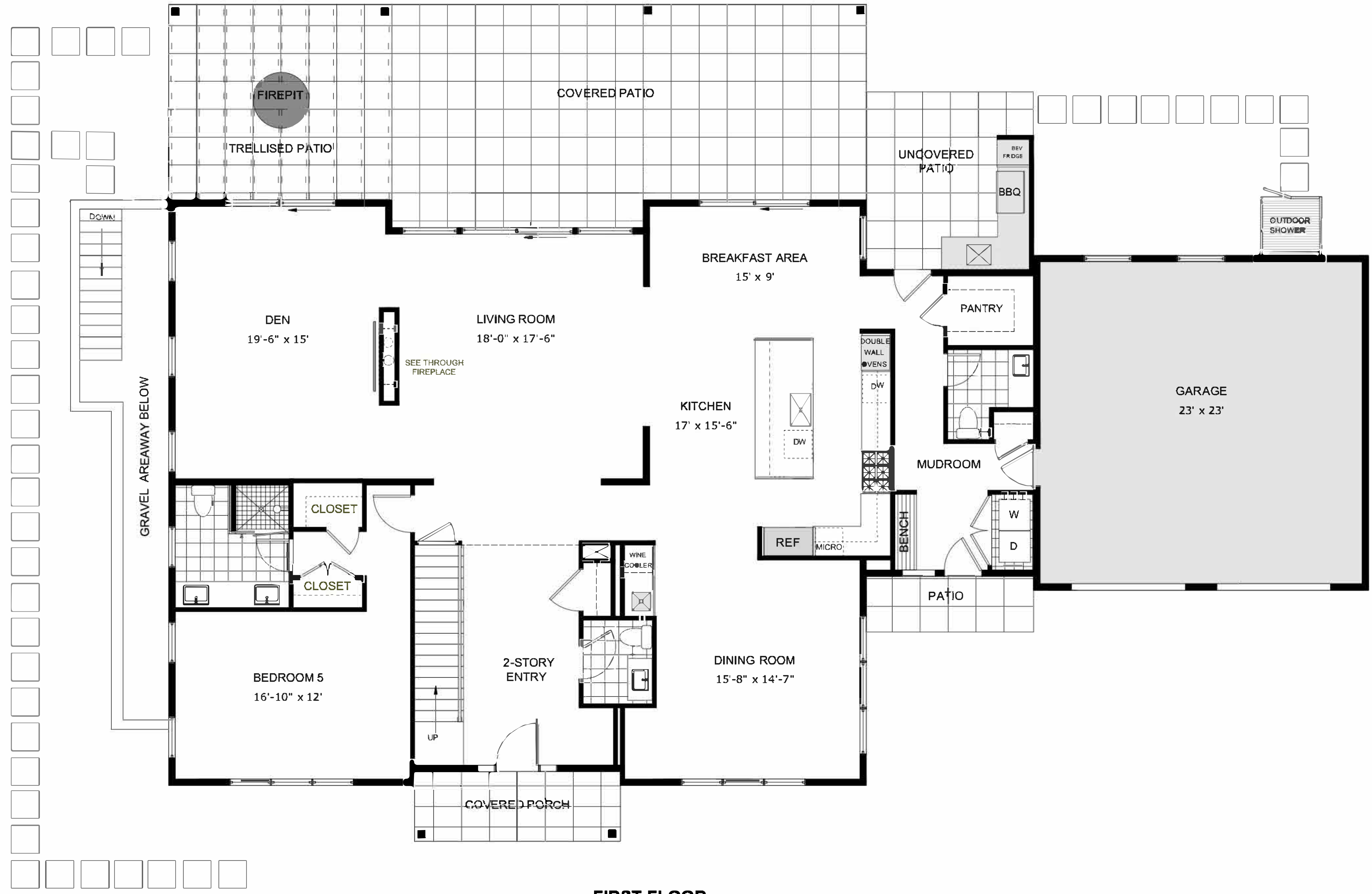
FIRST FLOOR
